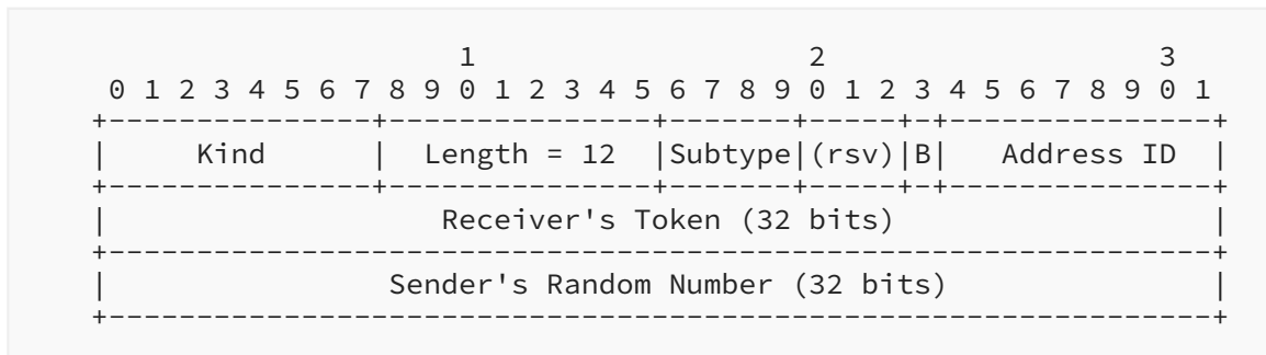
Figure 5: Join Connection (MP_JOIN) Option (for Initial SYN)
