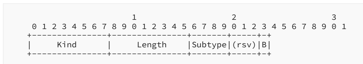
Figure 11: Change Subflow Priority (MP_PRIO) Option
